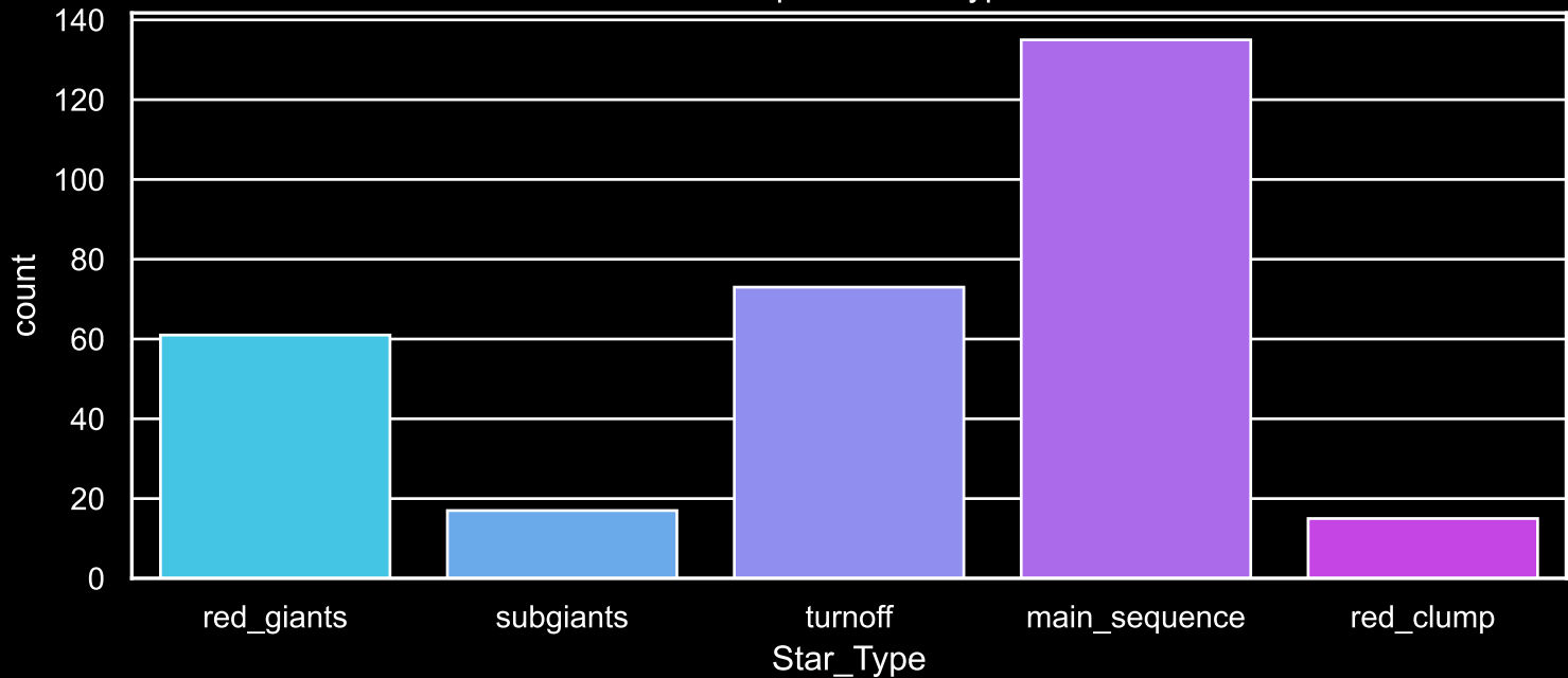
Field [73] Count plot of Star Type
