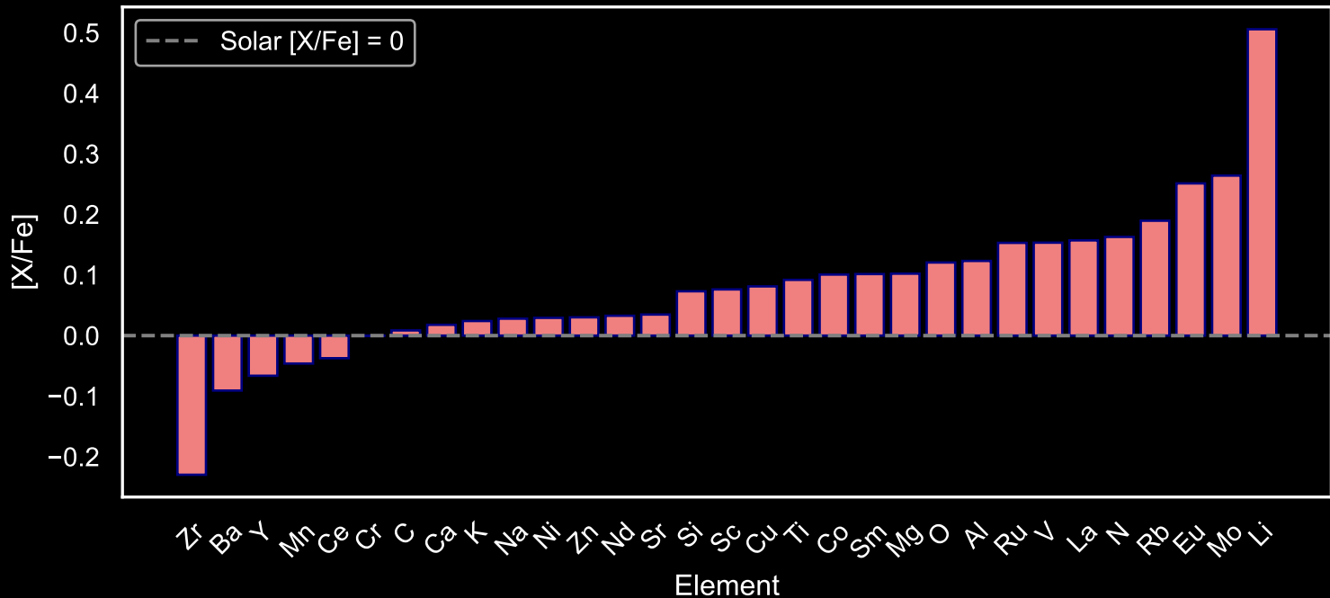
Abundance Pattern for GALAH Star Field [73] (N=301)
