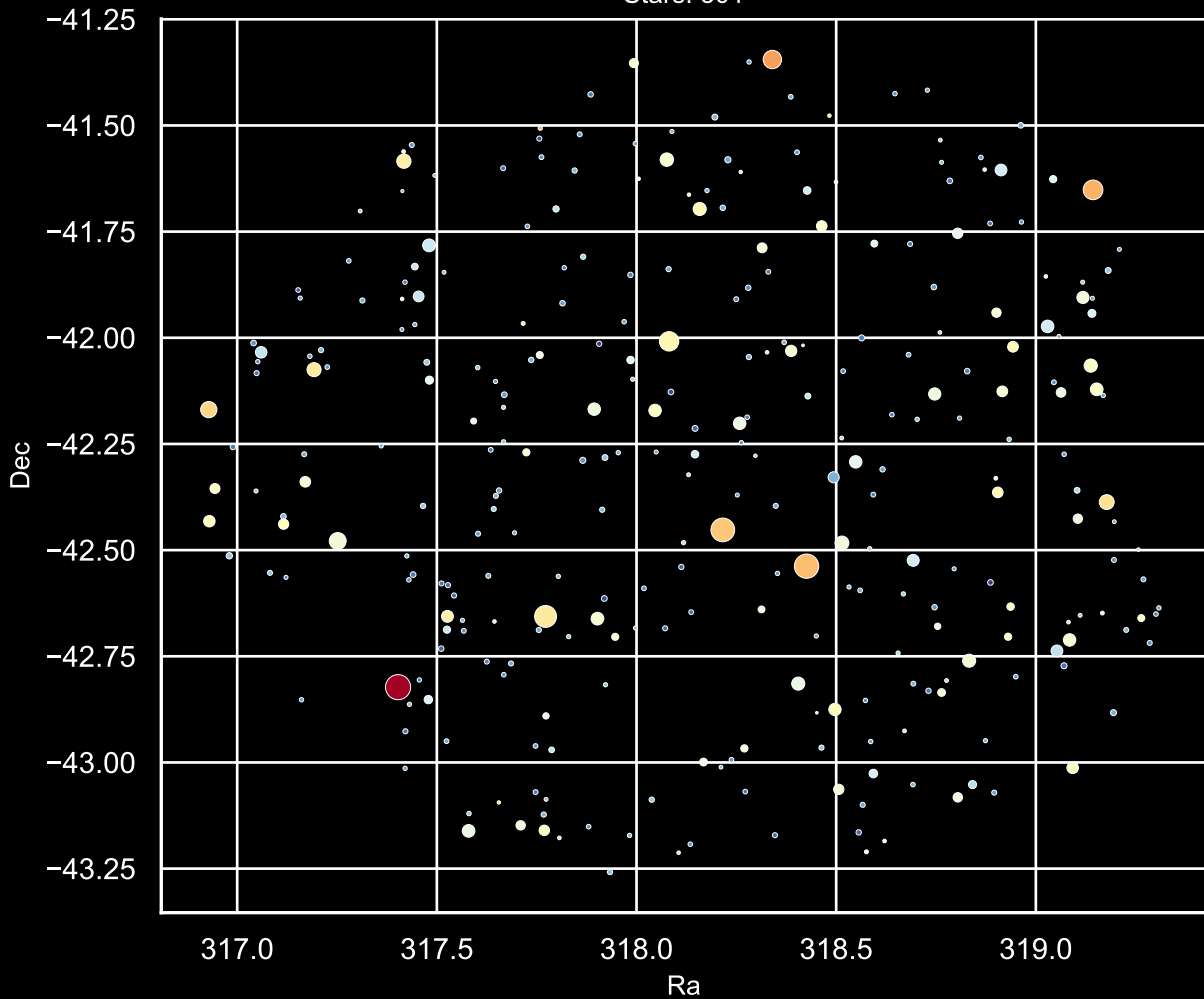
Field [73] Ra [318.17] Dec [-42.31] Stars: 301
