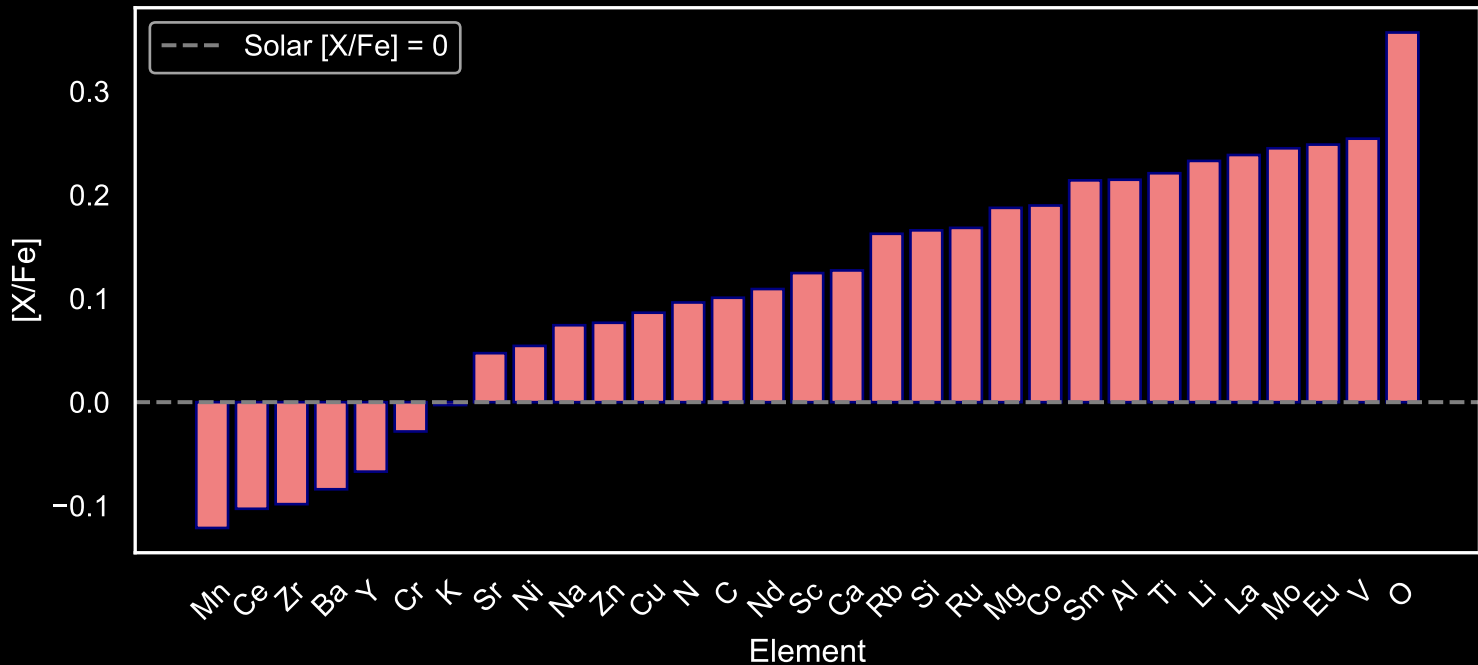
Abundance Pattern for GALAH Red Giants: Star Field [73] (N=76)
