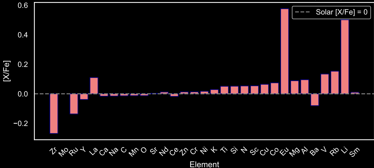
Abundance Pattern for GALAH Main Sequence Stars: Star Field [73] (N=135)
